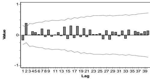
AR(1) - ACF, Significance limit (top), Significance limit (bottom)
