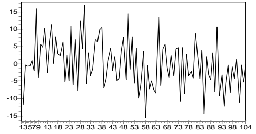
AR(1) - residuals
