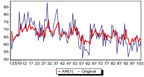
AR(1), Original copy
