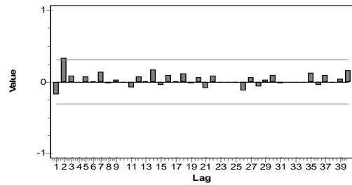
AR(1) - PACF, Significance limit (top), Significance limit (bottom)
