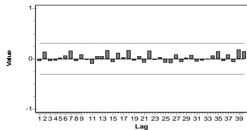
AR(2) - PACF, Significance limit (top), Significance limit (bottom)
