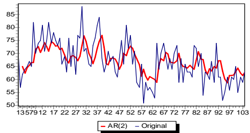
AR(2), Original copy
