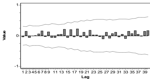
AR(2) - ACF, Significance limit (top), Significance limit (bottom)
