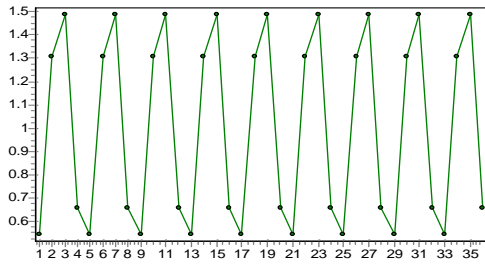
Seasonal factors (indices)
