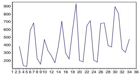
Trend and seasonal and random
