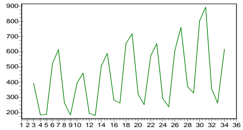
Trend and seasonal
